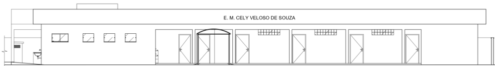
FACHADA PRINCIPAL ESCALA: 1/175
